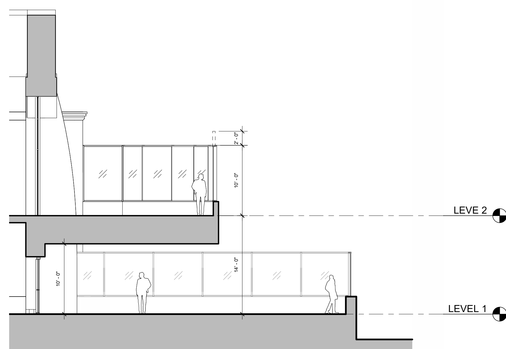
2 SECOND FLOOR TERRACE - SECTION 1/8" = 1'-0"
