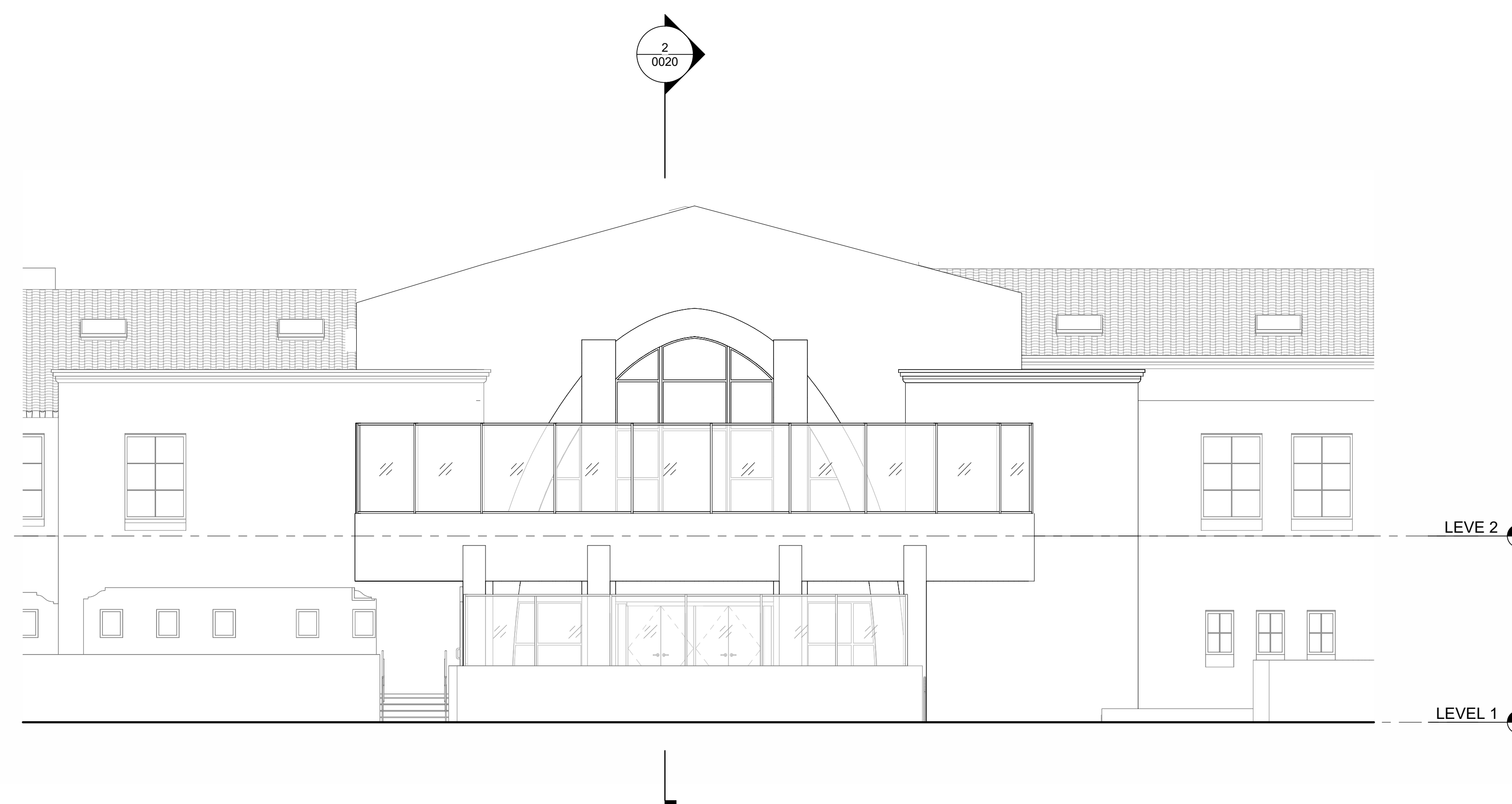
1 SECOND FLOOR TERRACE - WEST ELEVATION 1/8" = 1'-0"
