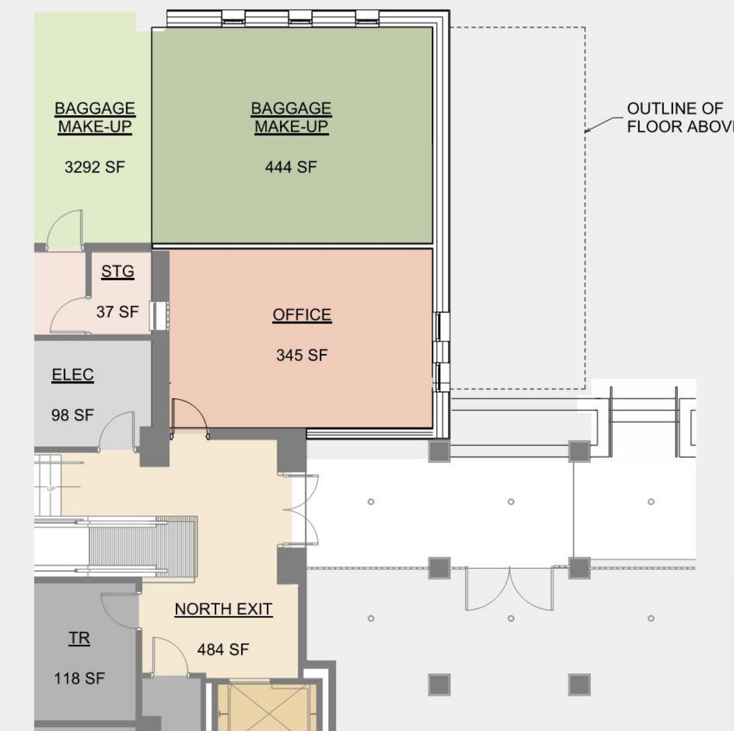
First Floor Plan- North End
