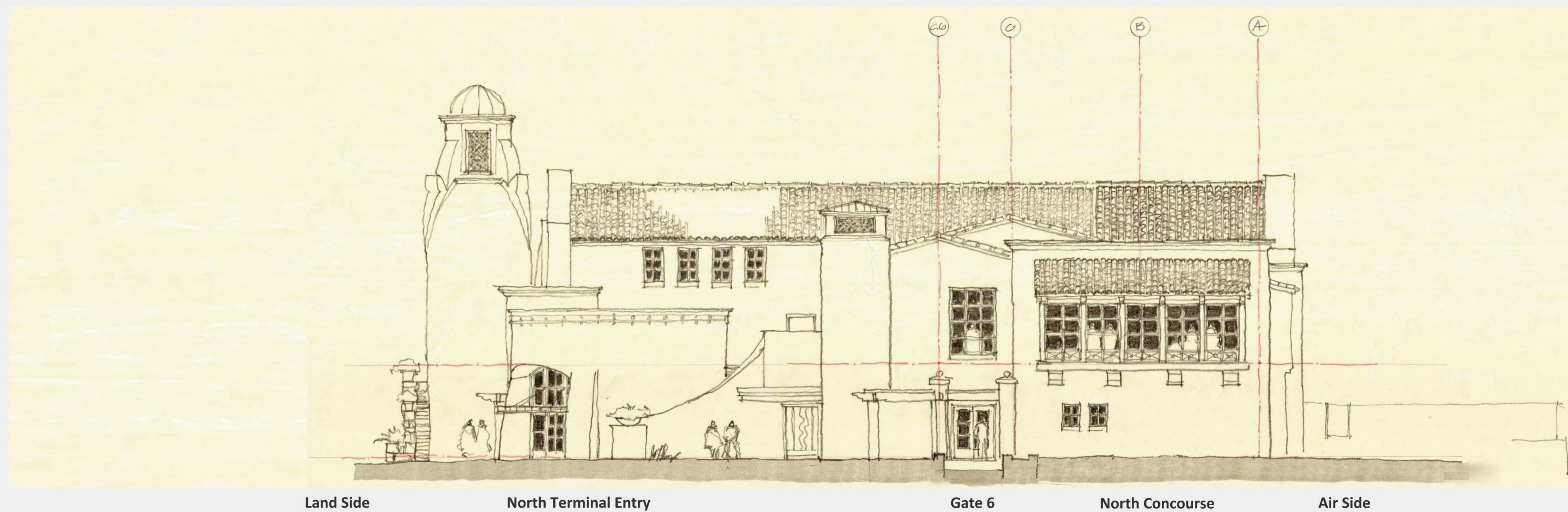
Air Side North Elevation
