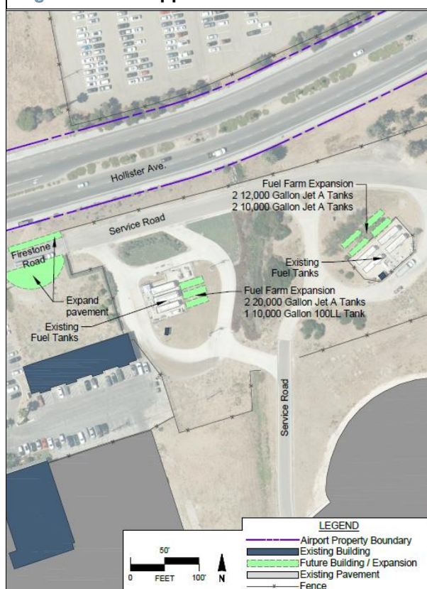
Figure 5-23: Support Facilities
