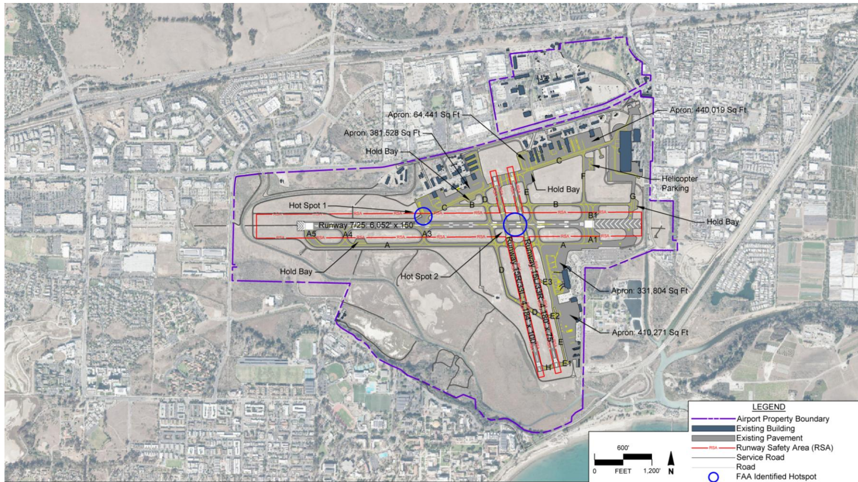
Figure 1-5: Airfield Runways and Taxiways
