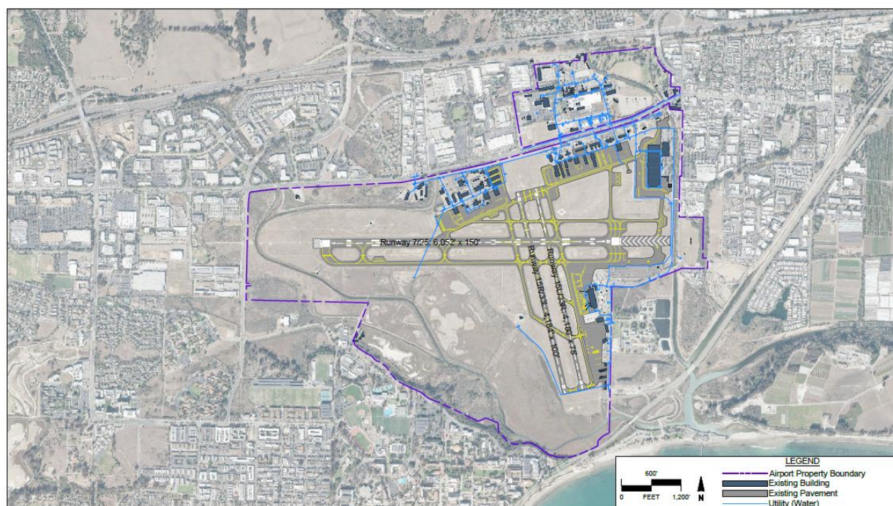
Figure 1-7: Figure 1: Santa Barbara Airport Water and Sewage Lines
